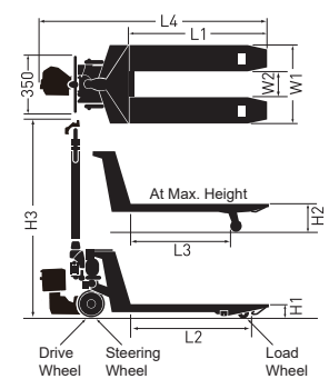
■ Dimensions (Standard Types)
