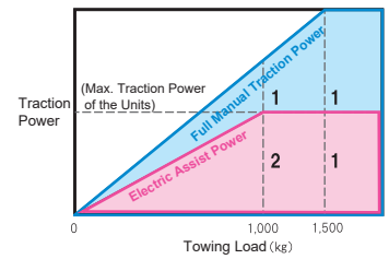
■ Assist Power Conceptual Diagram
