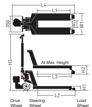
■ Dimensions (TCP Types)
